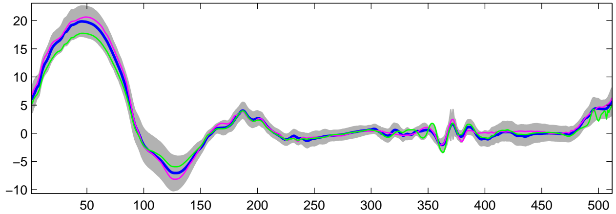
Estimated U_{22}(t) using G-WFMM: t_1 data, run 7
