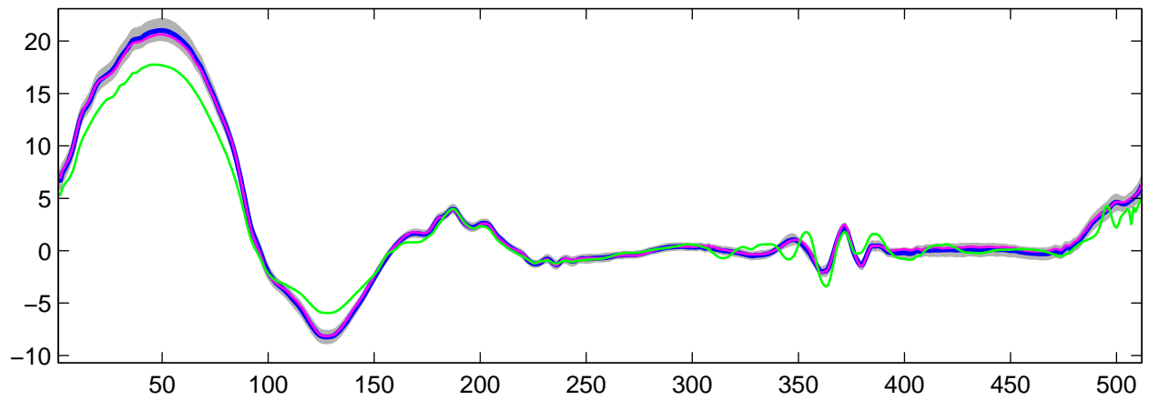
Estimated U_{22}(t) using R-WFMM: t_1 data, run 7
