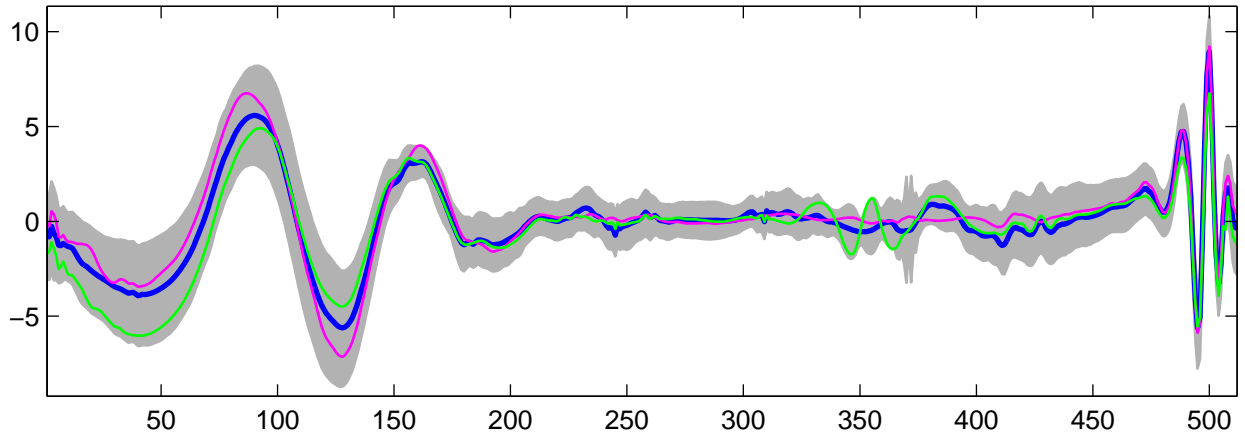
Estimated U_{23}(t) using G-WFMM: t_1 data, run 7
