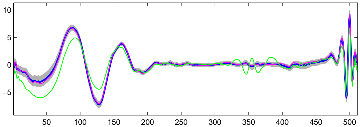
Estimated U_{23}(t) using R-WFMM: t_1 data, run 7
