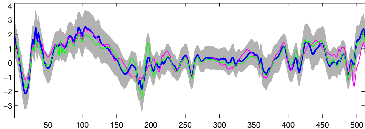
Estimated U_{23}(t) using G-WFMM: t_2 data, run 7
