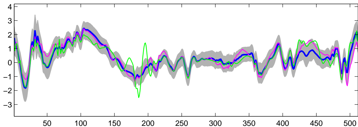
Estimated U_{23}(t) using R-WFMM: t_2 data, run 7
