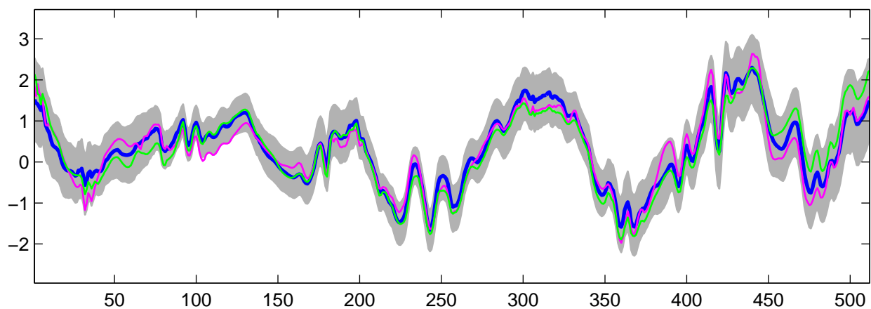
Estimated U_{25}(t) using R-WFMM: DE data, run 7
