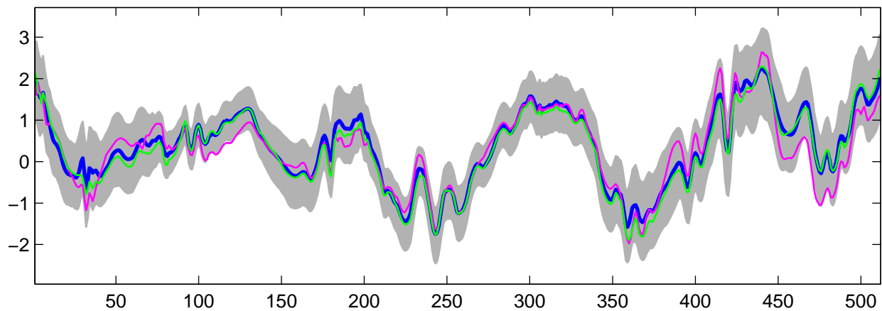
Estimated U_{25}(t) using G-WFMM: DE data, run 7
