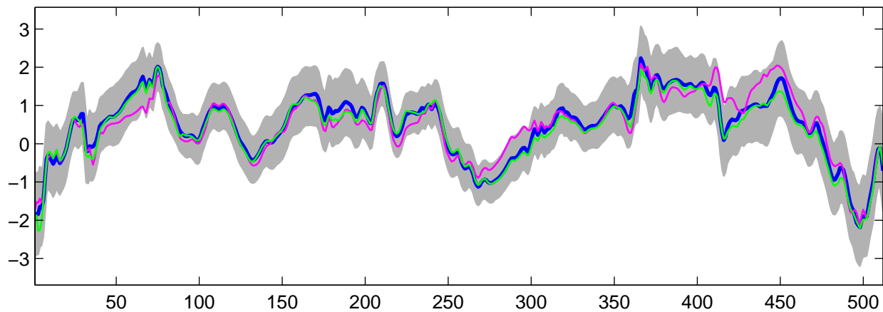
Estimated U_{25}(t) using G-WFMM: Normal data, run 7
