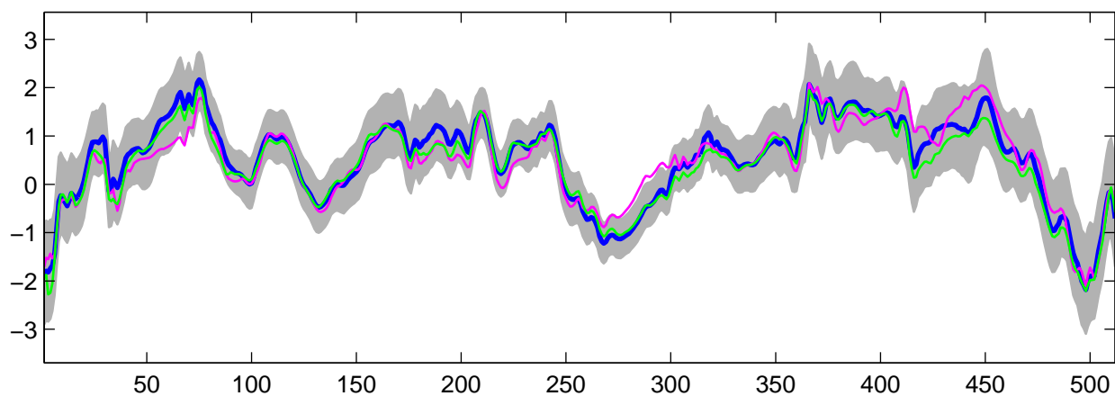
Estimated U_{25}(t) using R-WFMM: Normal data, run 7
