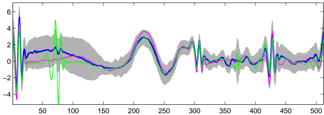
Estimated U_{25}(t) using G-WFMM: t_1 data, run 7
