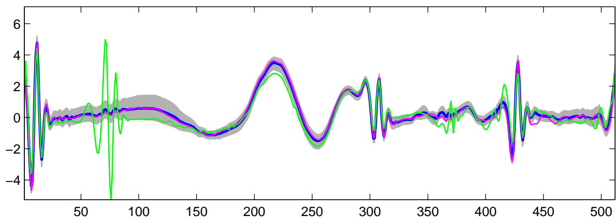
Estimated U_{25}(t) using R-WFMM: t_1 data, run 7
