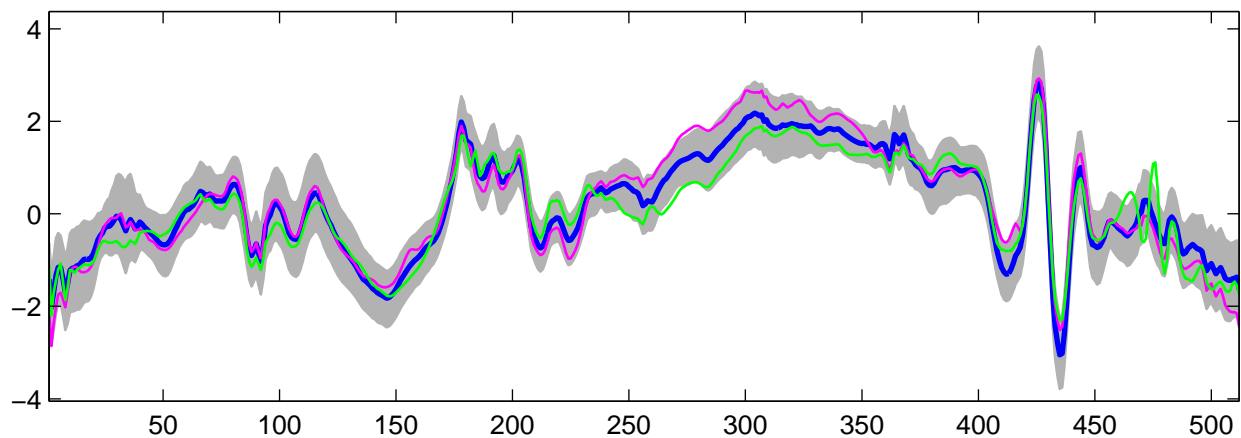
Estimated U_{25}(t) using R-WFMM: t_2 data, run 7
