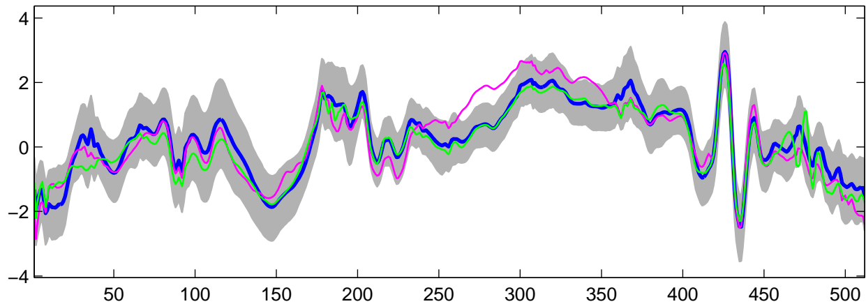
Estimated U_{25}(t) using G-WFMM: t_2 data, run 7
