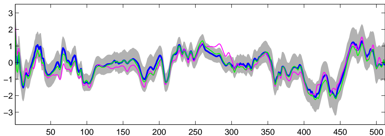
Estimated U_{26}(t) using R-WFMM: Normal data, run 7
