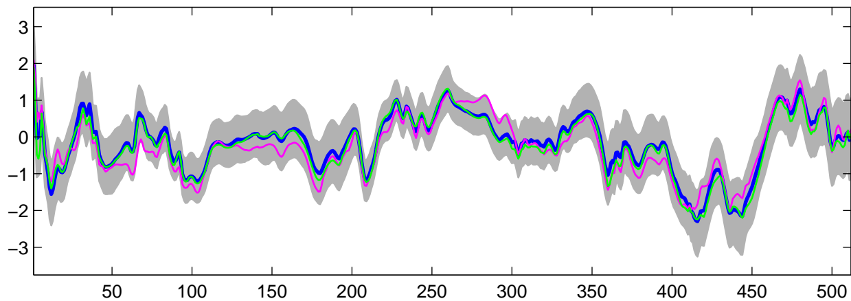
Estimated U_{26}(t) using G-WFMM: Normal data, run 7
