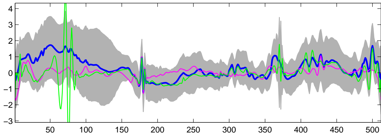
Estimated U_{26}(t) using G-WFMM: t_1 data, run 7
