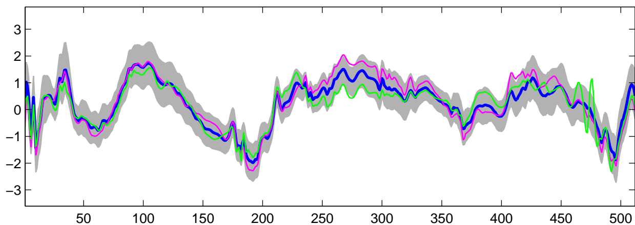
Estimated U_{26}(t) using R-WFMM: t_2 data, run 7
