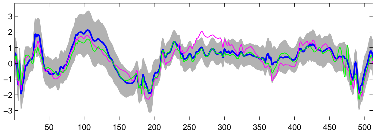
Estimated U_{26}(t) using G-WFMM: t_2 data, run 7
