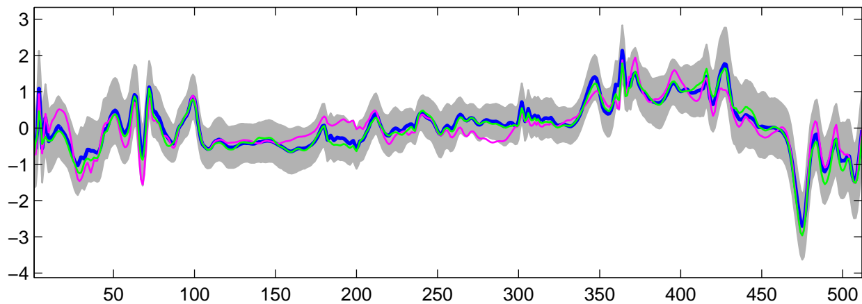
Estimated U_{26}(t) using G-WFMM: t_3 data, run 7
