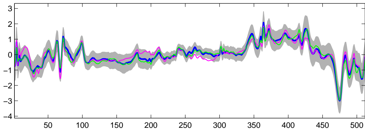
Estimated U_{26}(t) using R-WFMM: t_3 data, run 7
