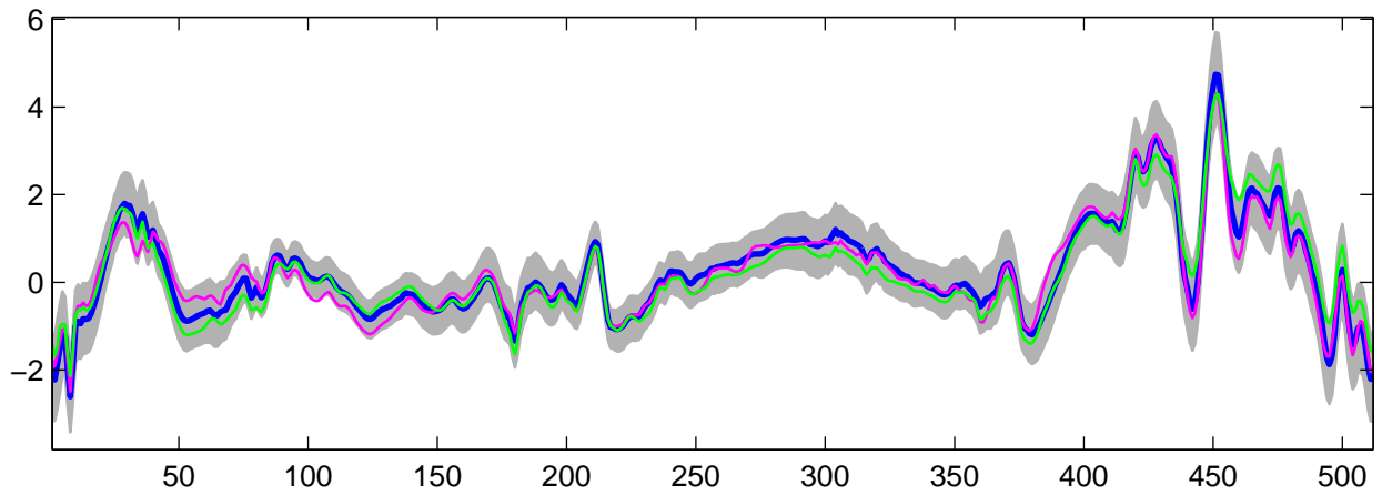
Estimated U_{27}(t) using R-WFMM: DE data, run 7
