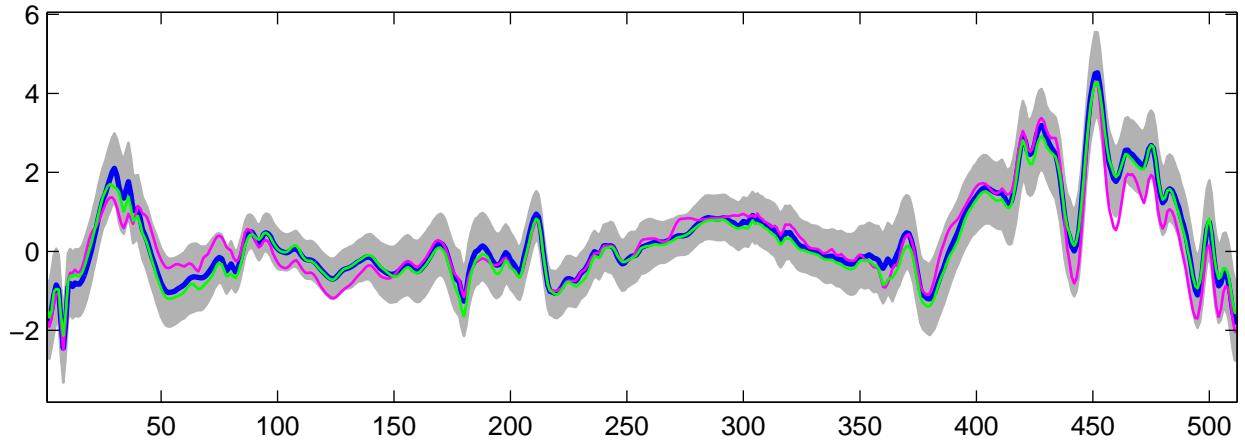
Estimated U_{27}(t) using G-WFMM: DE data, run 7
