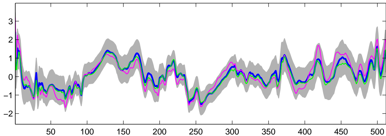
Estimated U_{27}(t) using G-WFMM: Normal data, run 7
