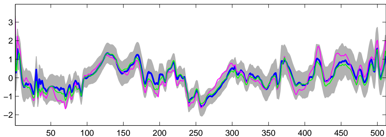
Estimated U_{27}(t) using R-WFMM: Normal data, run 7
