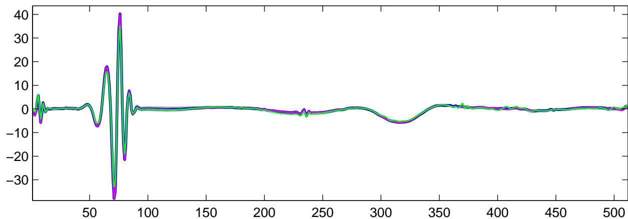
Estimated U_{27}(t) using R-WFMM: t_1 data, run 7
