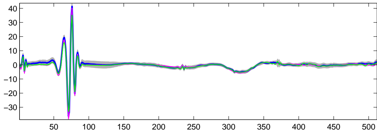
Estimated U_{27}(t) using G-WFMM: t_1 data, run 7
