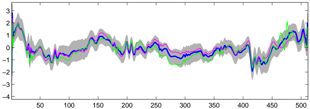
Estimated U_{27}(t) using R-WFMM: t_2 data, run 7
