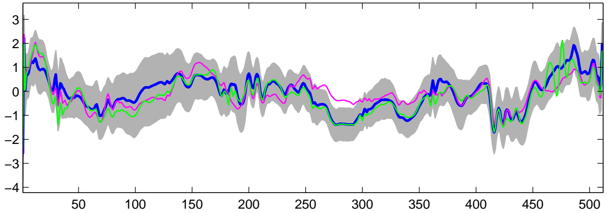
Estimated U_{27}(t) using G-WFMM: t_2 data, run 7
