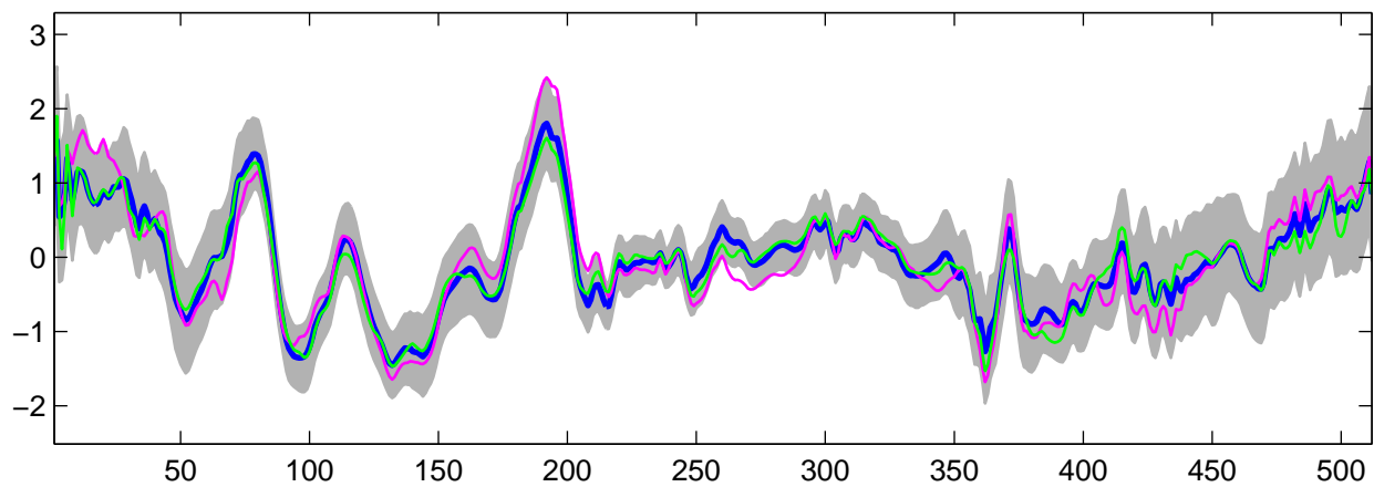
Estimated U_{27}(t) using R-WFMM: t_3 data, run 7
