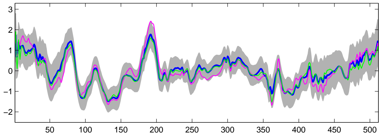
Estimated U_{27}(t) using G-WFMM: t_3 data, run 7
