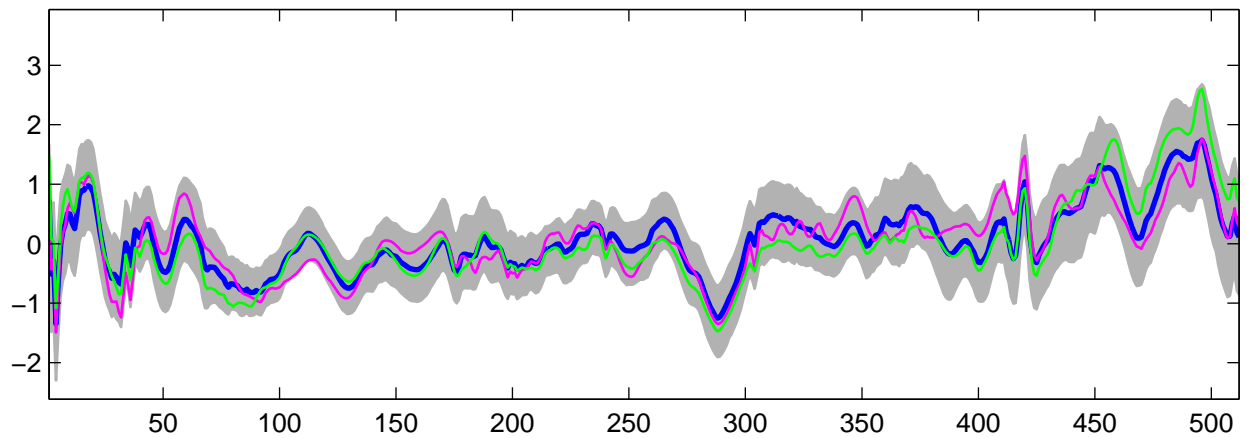
Estimated U_{28}(t) using R-WFMM: DE data, run 7
