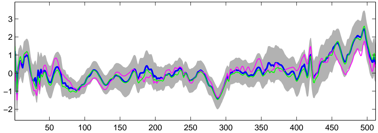
Estimated U_{28}(t) using G-WFMM: DE data, run 7
