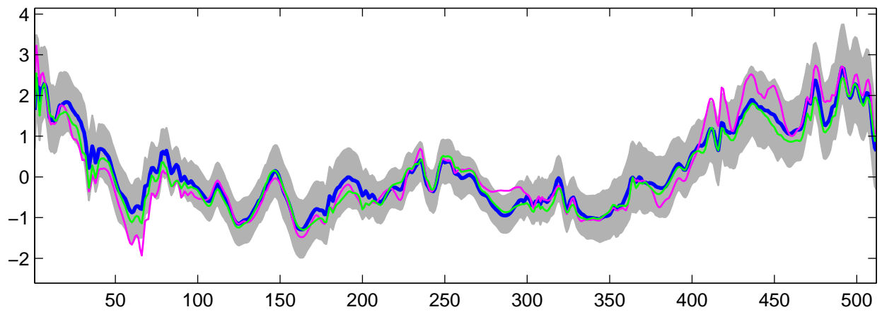
Estimated U_{28}(t) using R-WFMM: Normal data, run 7
