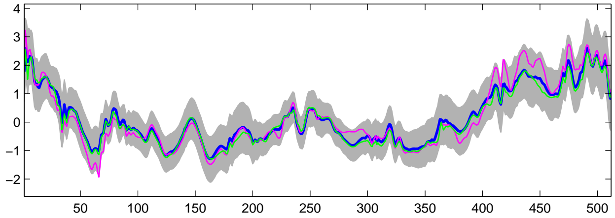
Estimated U_{28}(t) using G-WFMM: Normal data, run 7
