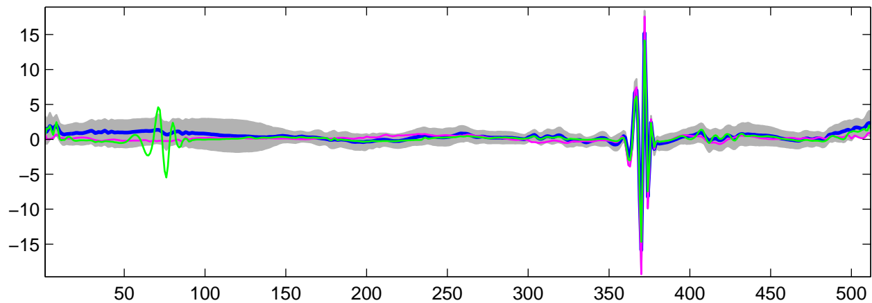
Estimated U_{28}(t) using G-WFMM: t_1 data, run 7
