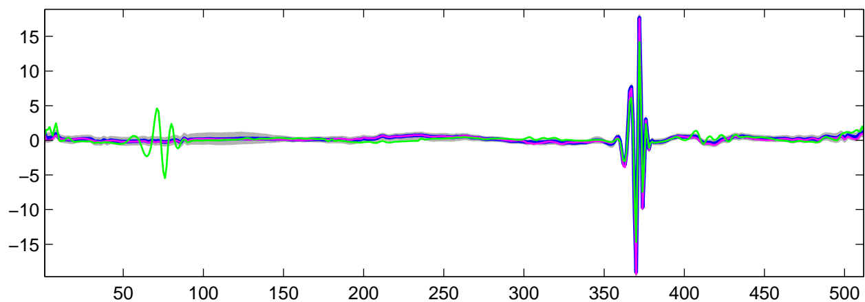
Estimated U_{28}(t) using R-WFMM: t_1 data, run 7
