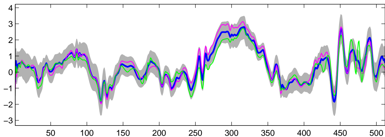
Estimated U_{28}(t) using R-WFMM: t_2 data, run 7
