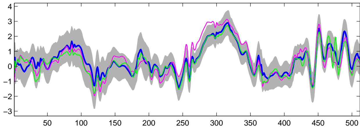
Estimated U_{28}(t) using G-WFMM: t_2 data, run 7
