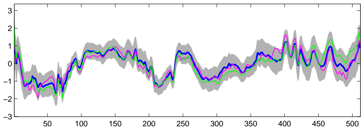
Estimated U_{29}(t) using R-WFMM: DE data, run 7
