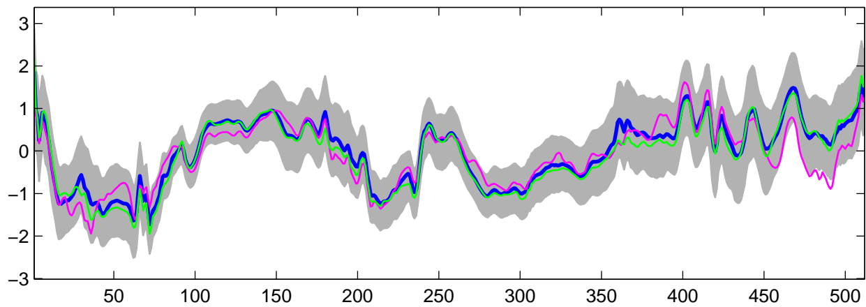
Estimated U_{29}(t) using G-WFMM: DE data, run 7
