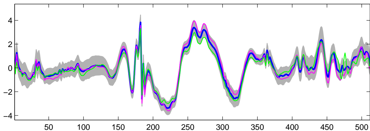
Estimated U_{29}(t) using R-WFMM: t_2 data, run 7
