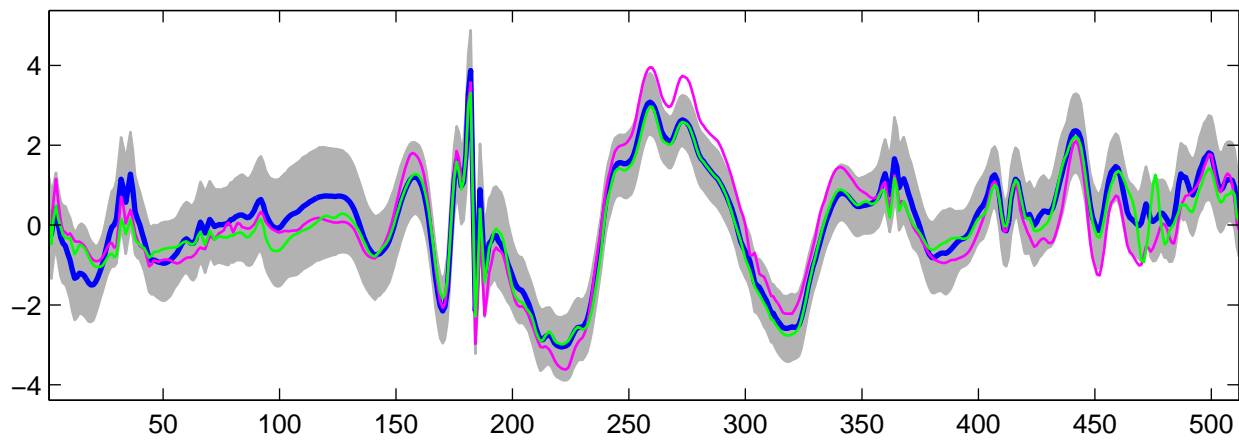
Estimated U_{29}(t) using G-WFMM: t_2 data, run 7
