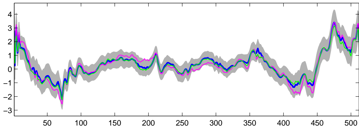
Estimated U_{29}(t) using G-WFMM: t_3 data, run 7
