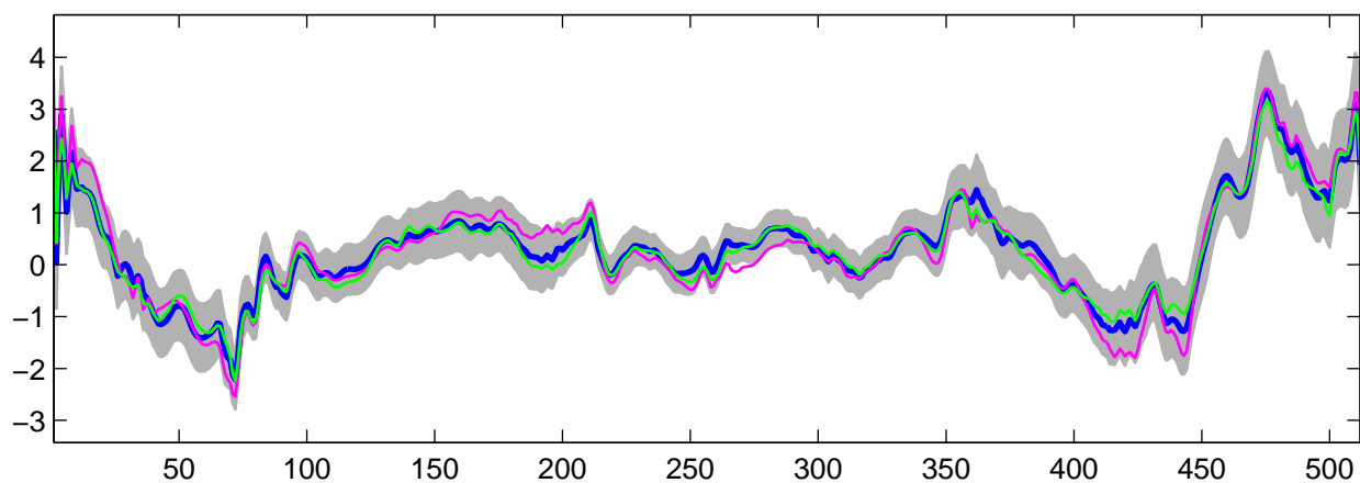
Estimated U_{29}(t) using R-WFMM: t_3 data, run 7
