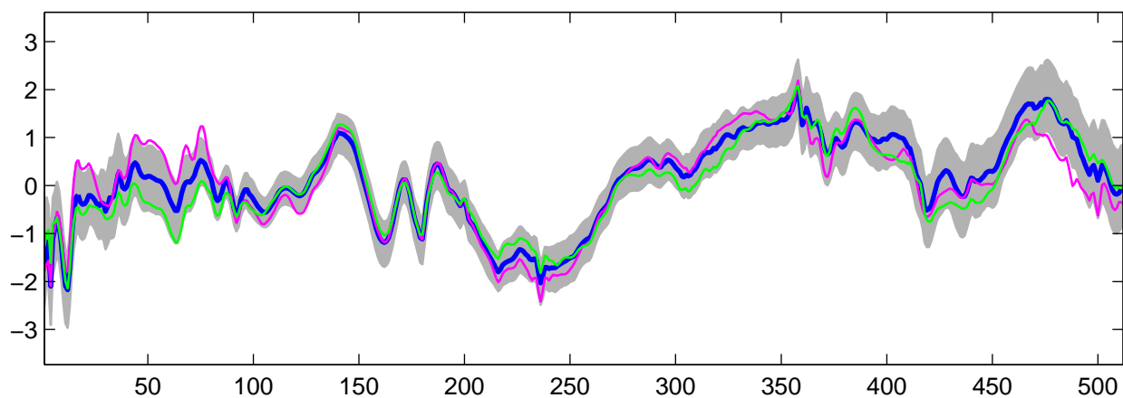
Estimated U_2(t) using R-WFMM: DE data, run 7
