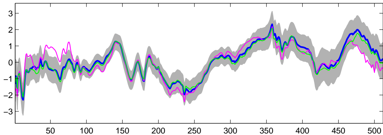
Estimated U_2(t) using G-WFMM: DE data, run 7
