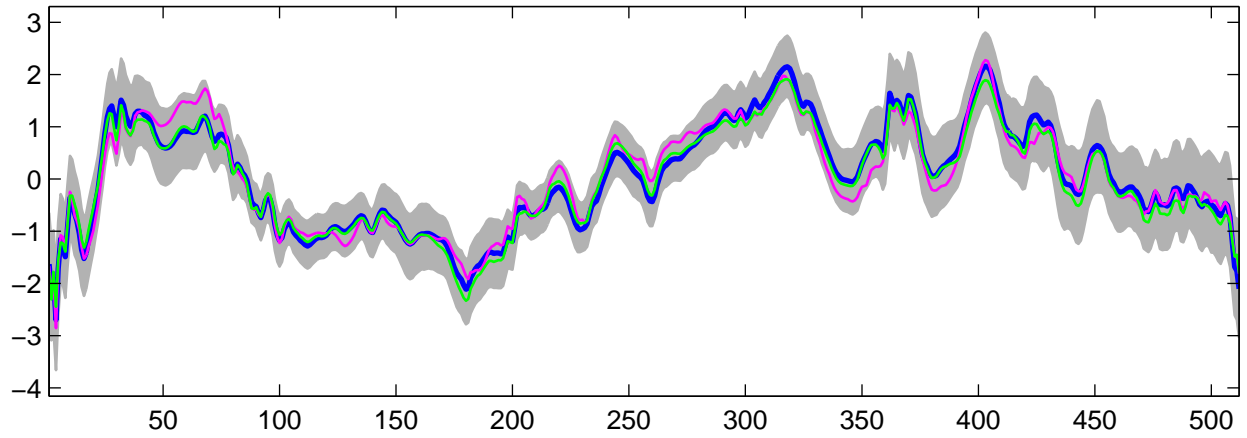
Estimated U_2(t) using G-WFMM: Normal data, run 7
