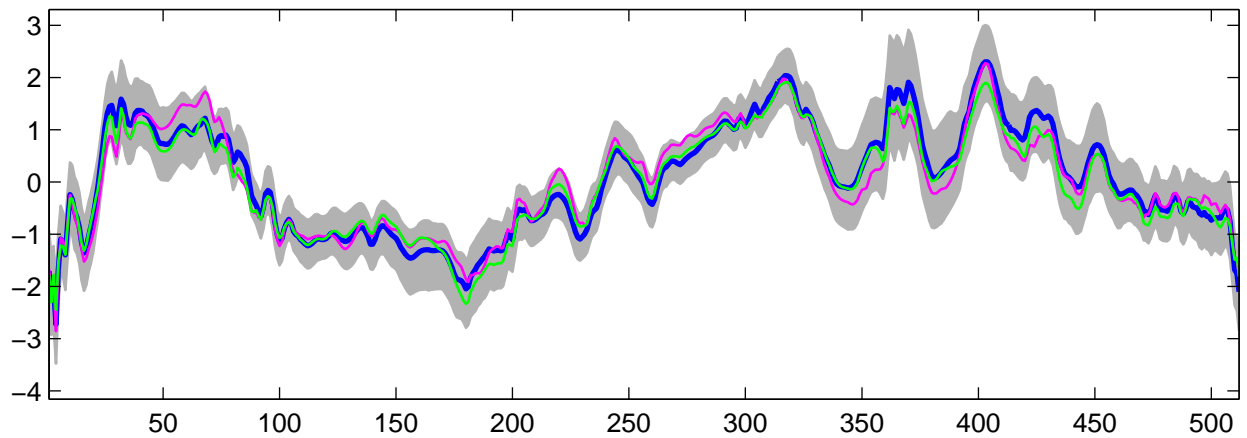
Estimated U_2(t) using R-WFMM: Normal data, run 7
