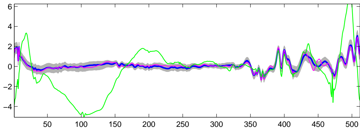
Estimated U_2(t) using R-WFMM: t_1 data, run 7
