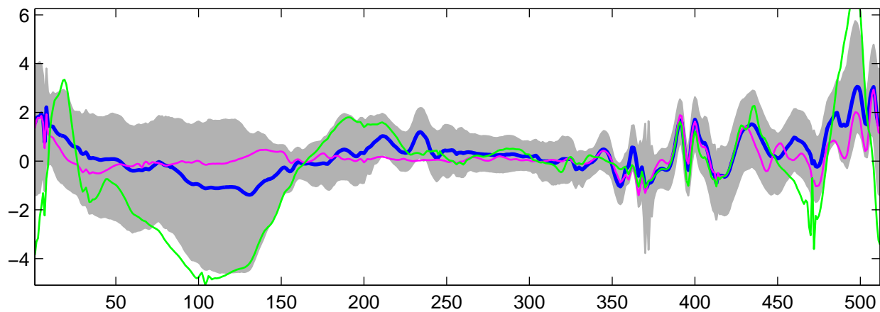
Estimated U_2(t) using G-WFMM: t_1 data, run 7
