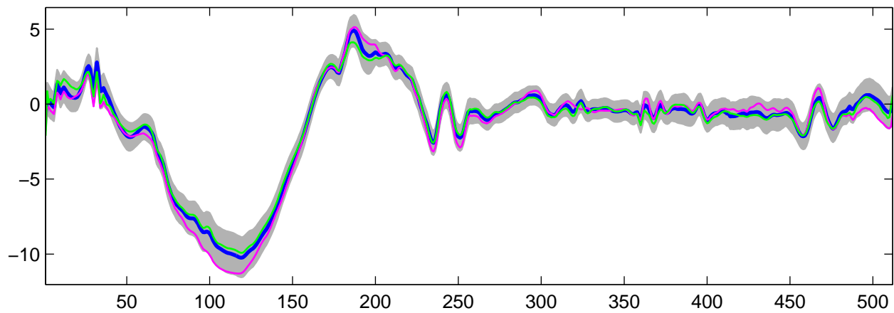
Estimated U_2(t) using G-WFMM: t_2 data, run 7
