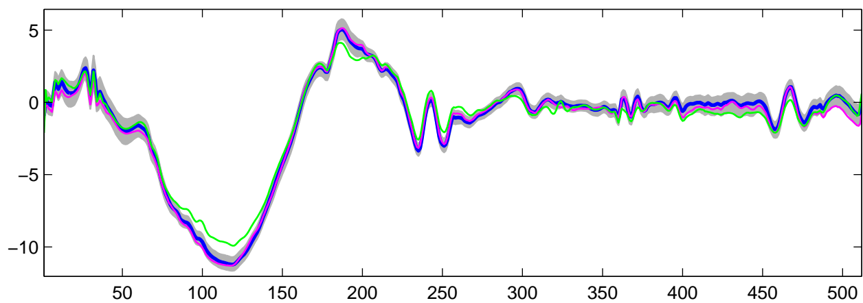
Estimated U_2(t) using R-WFMM: t_2 data, run 7
