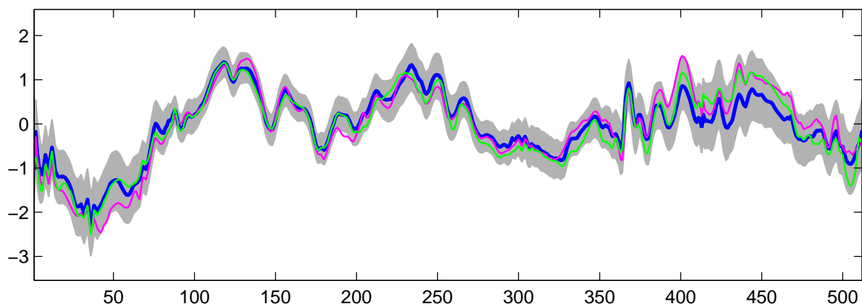
Estimated U_2(t) using R-WFMM: t_3 data, run 7
