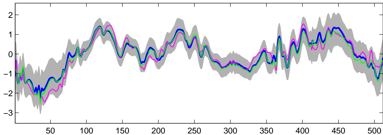
Estimated U_2(t) using G-WFMM: t_3 data, run 7
