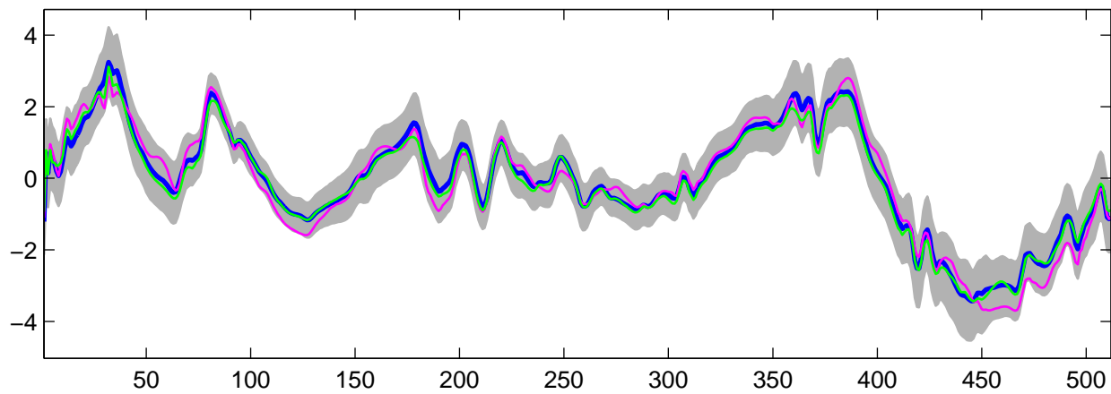
Estimated U_{30}(t) using G-WFMM: DE data, run 7
