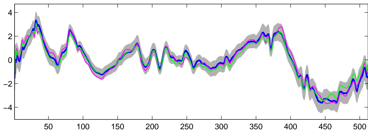
Estimated U_{30}(t) using R-WFMM: DE data, run 7
