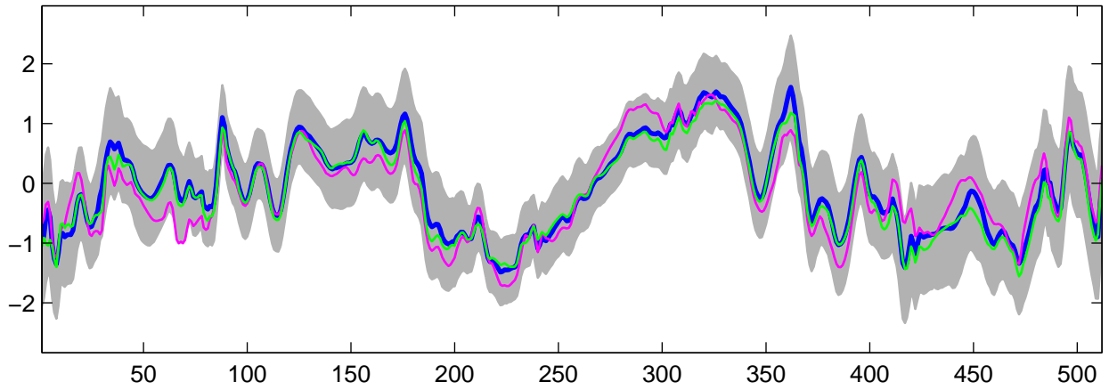
Estimated U_{30}(t) using G-WFMM: Normal data, run 7
