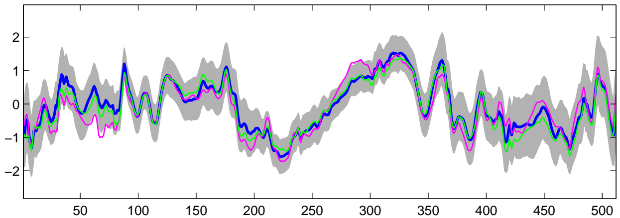
Estimated U_{30}(t) using R-WFMM: Normal data, run 7
