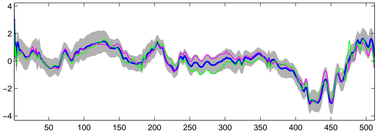
Estimated U_{30}(t) using R-WFMM: t_2 data, run 7
