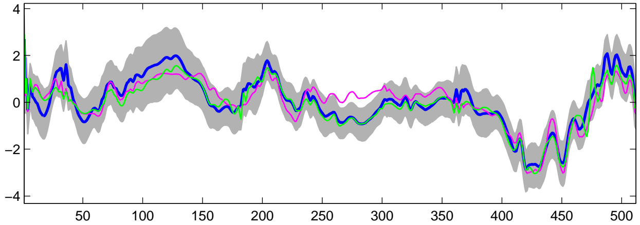
Estimated U_{30}(t) using G-WFMM: t_2 data, run 7
