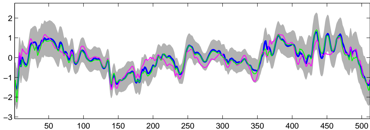
Estimated U_{30}(t) using G-WFMM: t_3 data, run 7
