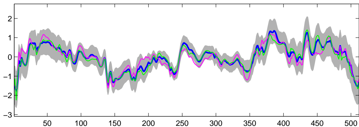
Estimated U_{30}(t) using R-WFMM: t_3 data, run 7
