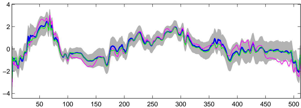
Estimated U_{31}(t) using G-WFMM: DE data, run 7
