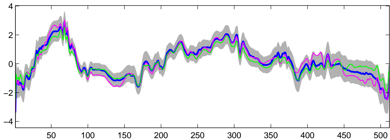
Estimated U_{31}(t) using R-WFMM: DE data, run 7
