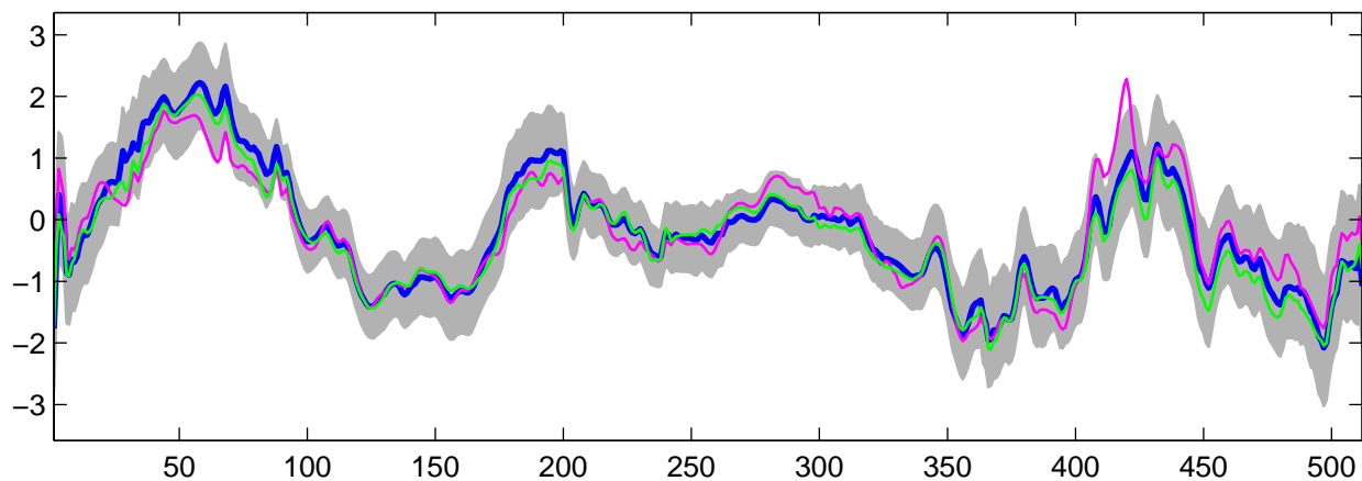
Estimated U_{31}(t) using R-WFMM: Normal data, run 7
