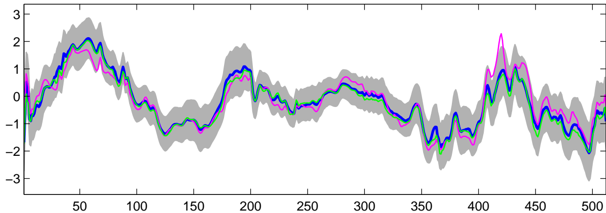
Estimated U_{31}(t) using G-WFMM: Normal data, run 7
