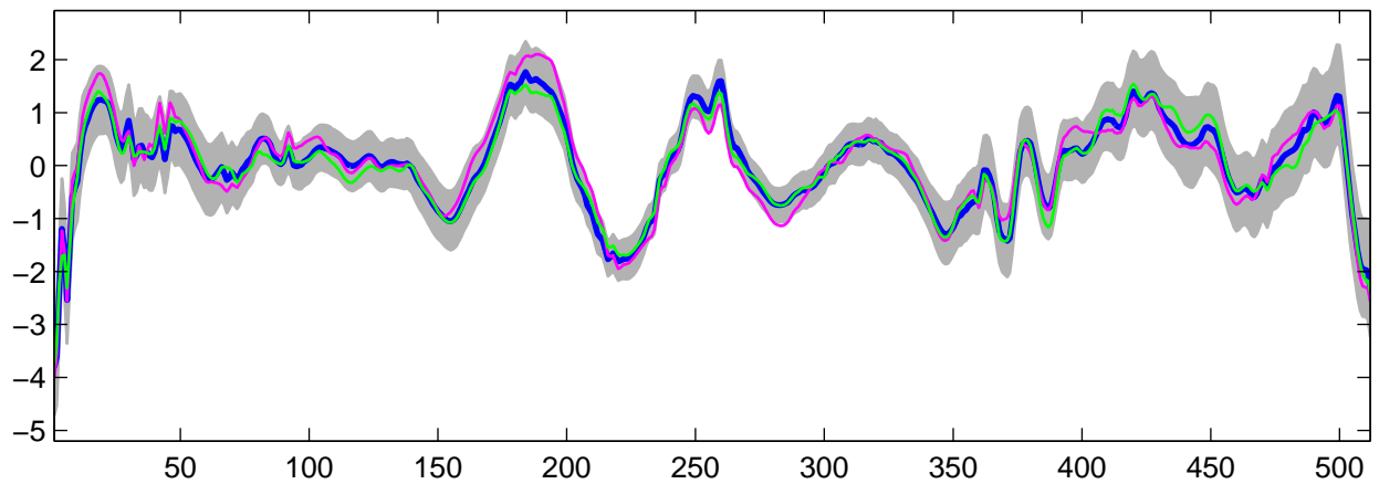
Estimated U_{31}(t) using R-WFMM: t_3 data, run 7
