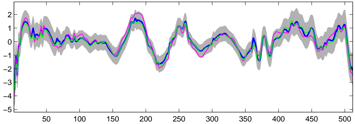
Estimated U_{31}(t) using G-WFMM: t_3 data, run 7
