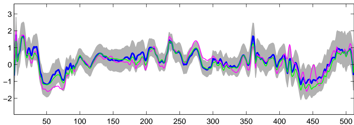
Estimated U_{32}(t) using R-WFMM: Normal data, run 7
