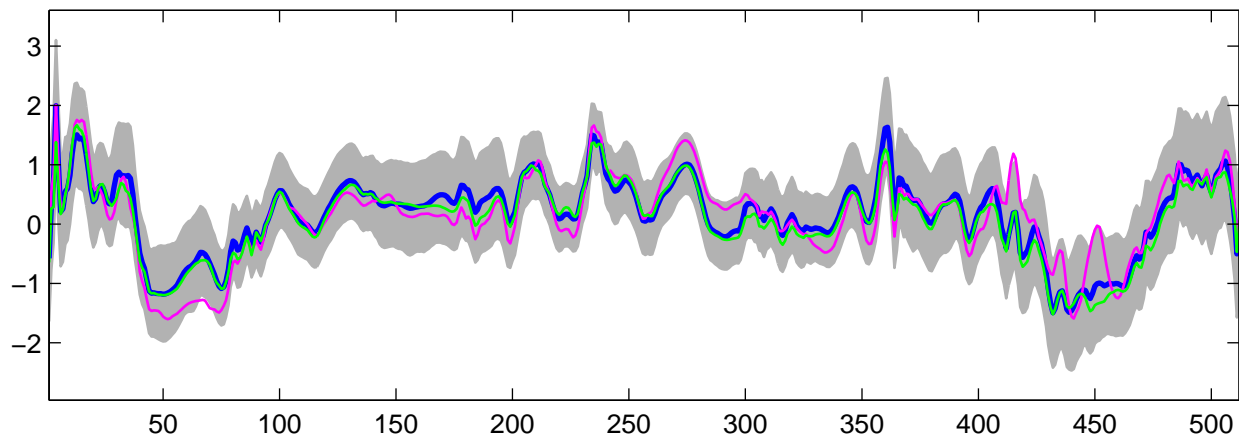
Estimated U_{32}(t) using G-WFMM: Normal data, run 7
