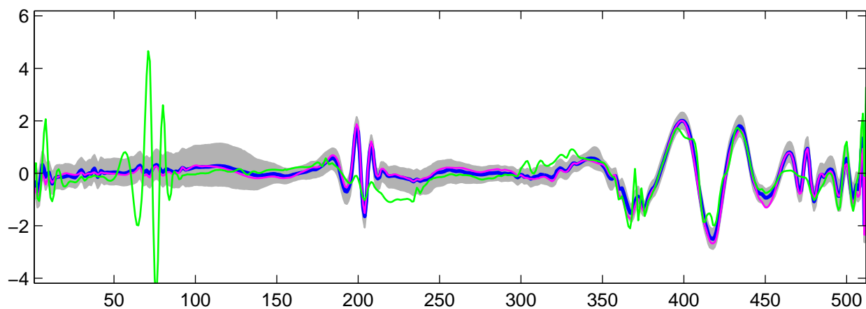
Estimated U_{32}(t) using R-WFMM: t_1 data, run 7
