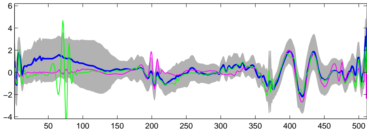
Estimated U_{32}(t) using G-WFMM: t_1 data, run 7
