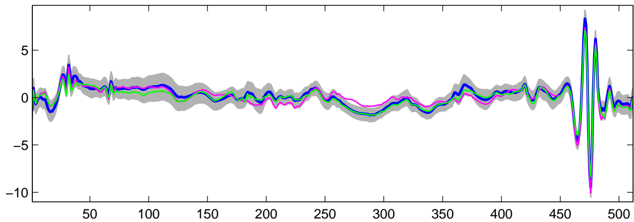
Estimated U_{32}(t) using G-WFMM: t_2 data, run 7
