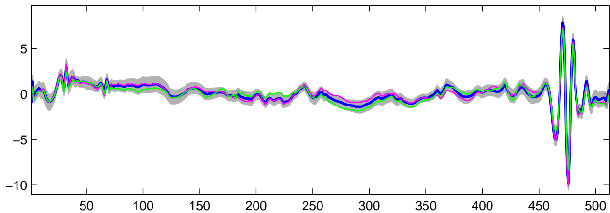
Estimated U_{32}(t) using R-WFMM: t_2 data, run 7
