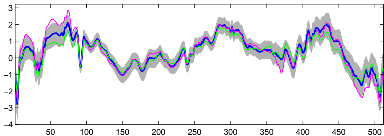
Estimated U_3(t) using R-WFMM: DE data, run 7
