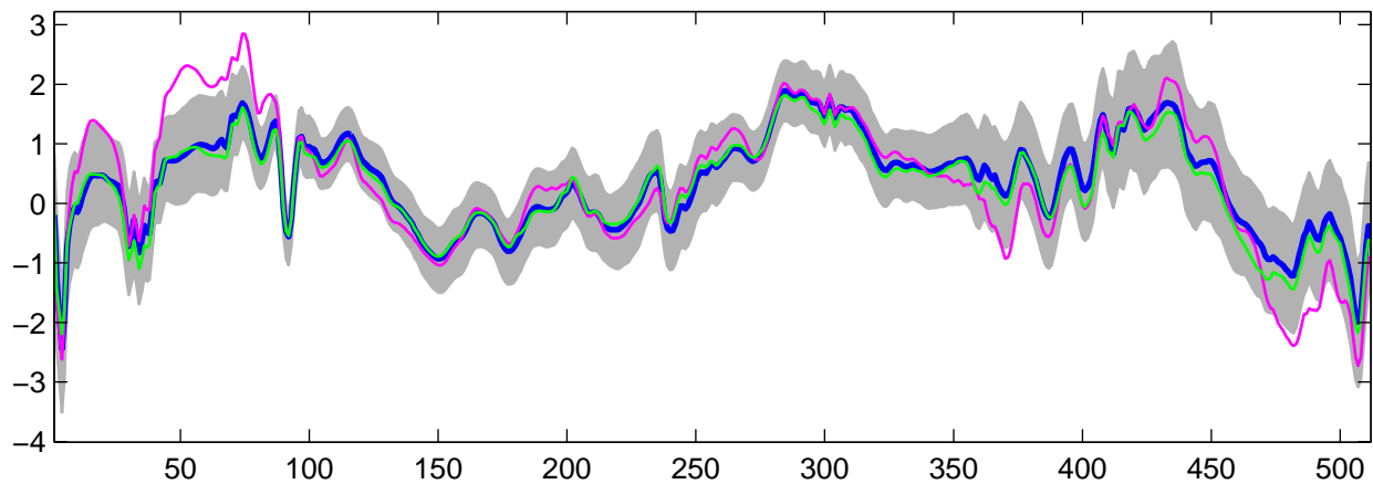
Estimated U_3(t) using G-WFMM: DE data, run 7
