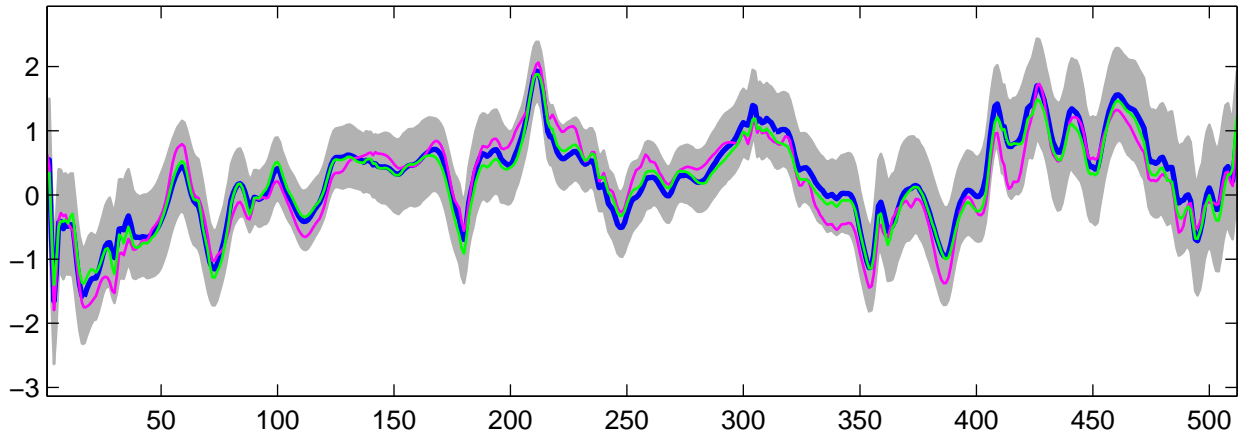
Estimated U_3(t) using G-WFMM: Normal data, run 7
