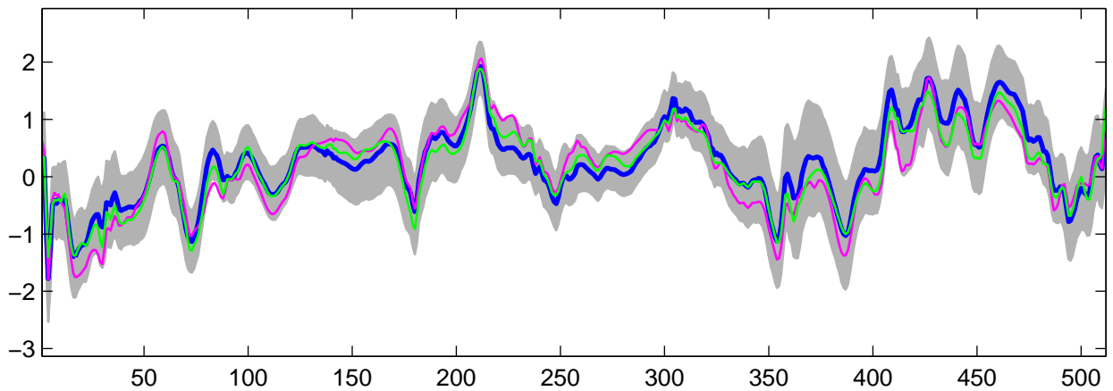
Estimated U_3(t) using R-WFMM: Normal data, run 7
