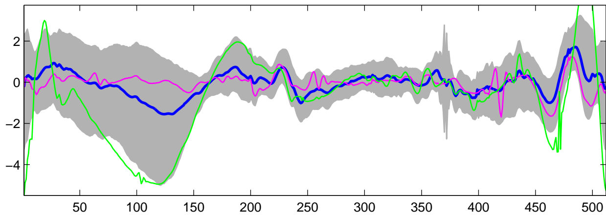
Estimated U_3(t) using G-WFMM: t_1 data, run 7
