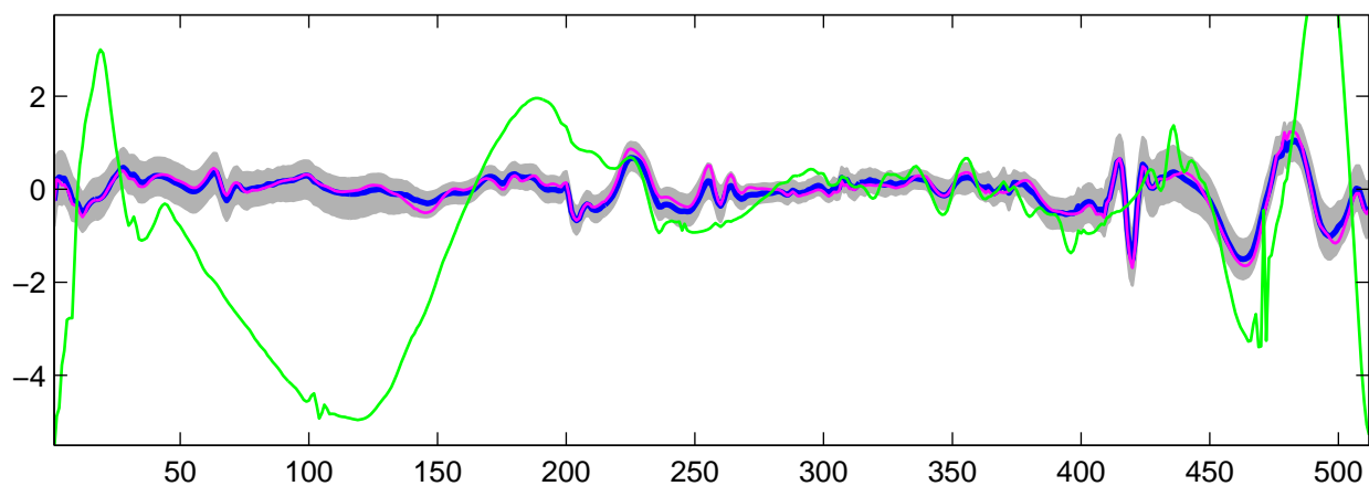
Estimated U_3(t) using R-WFMM: t_1 data, run 7
