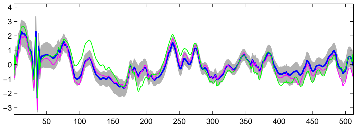
Estimated U_3(t) using R-WFMM: t_2 data, run 7
