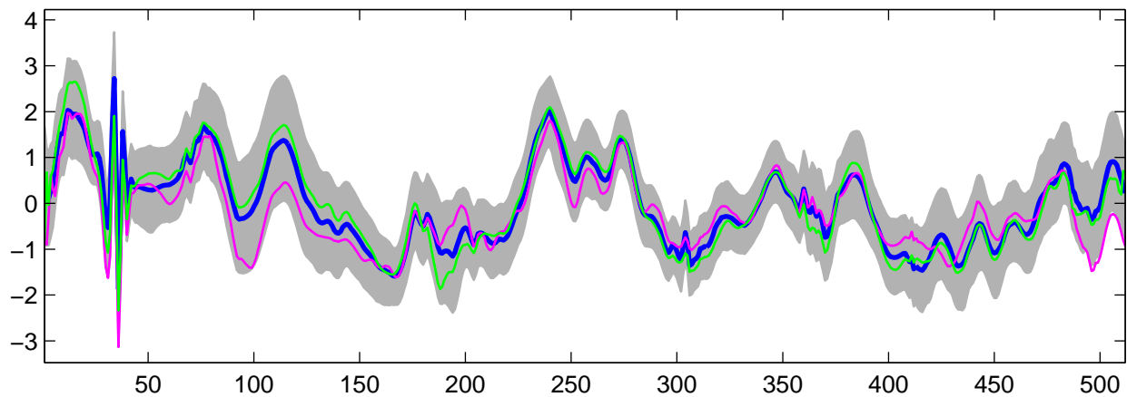
Estimated U_3(t) using G-WFMM: t_2 data, run 7
