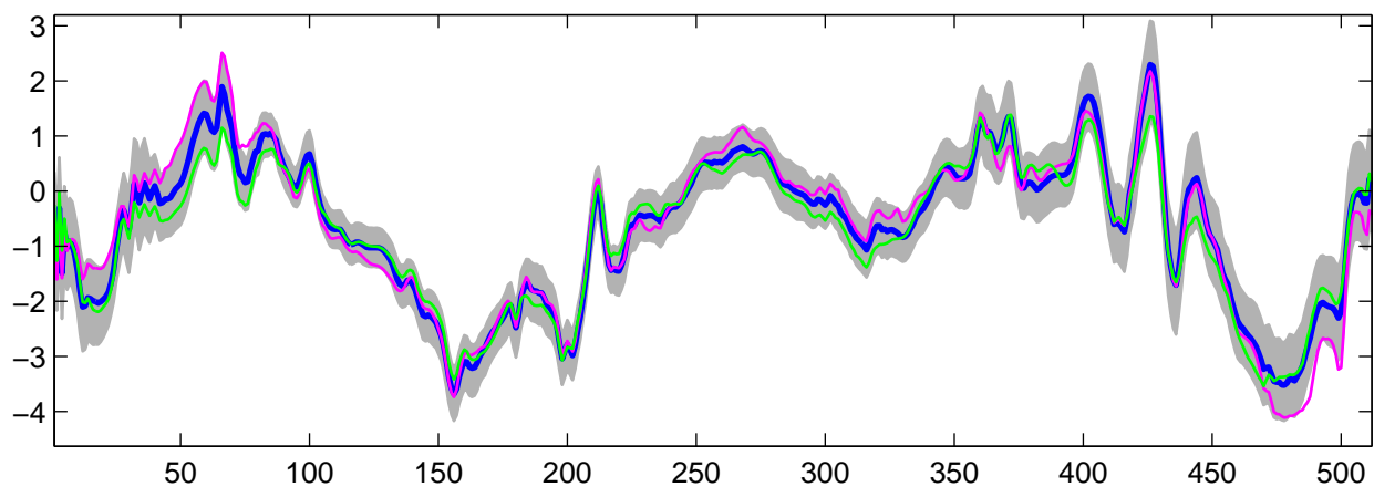
Estimated U_4(t) using R-WFMM: DE data, run 7
