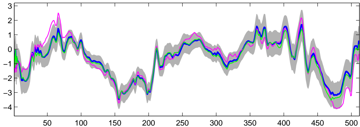
Estimated U_4(t) using G-WFMM: DE data, run 7
