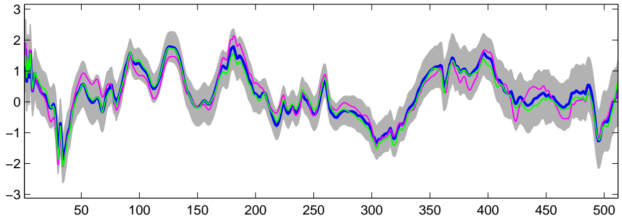
Estimated U_4(t) using G-WFMM: Normal data, run 7
