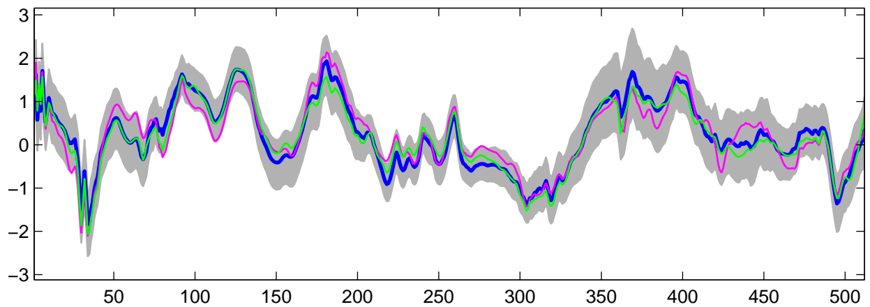
Estimated U_4(t) using R-WFMM: Normal data, run 7
