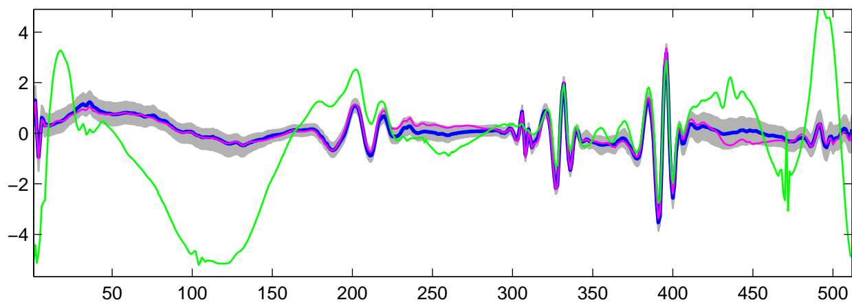
Estimated U_4(t) using R-WFMM: t_1 data, run 7
