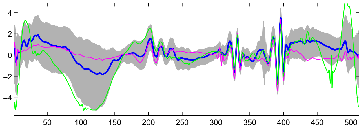
Estimated U_4(t) using G-WFMM: t_1 data, run 7
