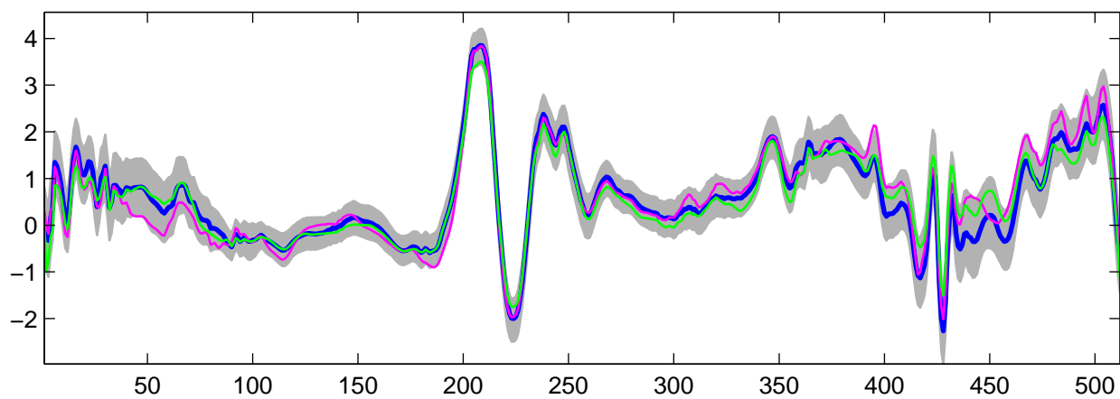
Estimated U_4(t) using R-WFMM: t_3 data, run 7
