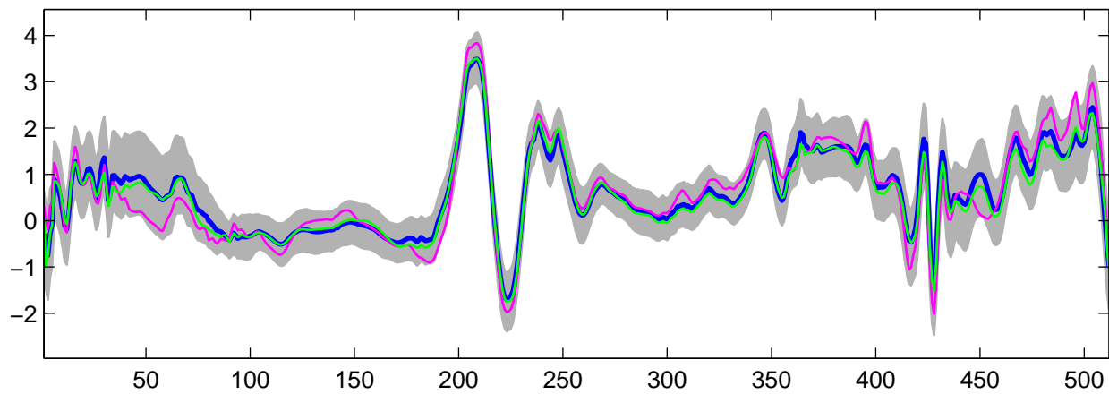
Estimated U_4(t) using G-WFMM: t_3 data, run 7
