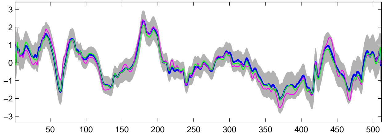
Estimated U_5(t) using G-WFMM: Normal data, run 7
