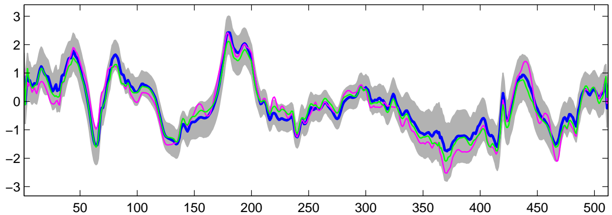
Estimated U_5(t) using R-WFMM: Normal data, run 7
