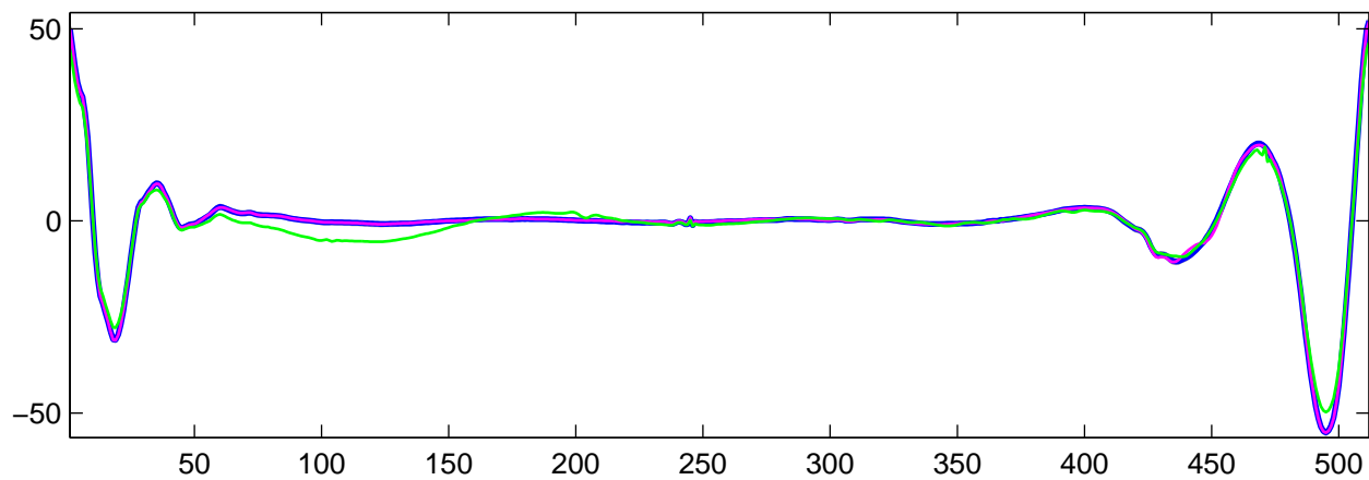
Estimated U_5(t) using R-WFMM: t_1 data, run 7
