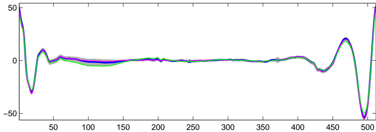
Estimated U_5(t) using G-WFMM: t_1 data, run 7
