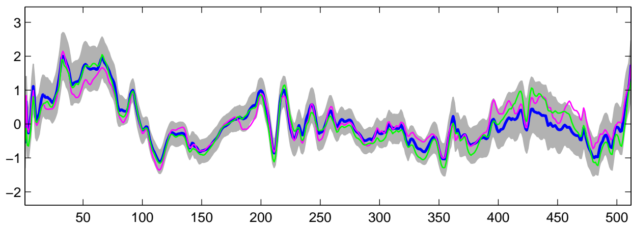
Estimated U_5(t) using R-WFMM: t_3 data, run 7
