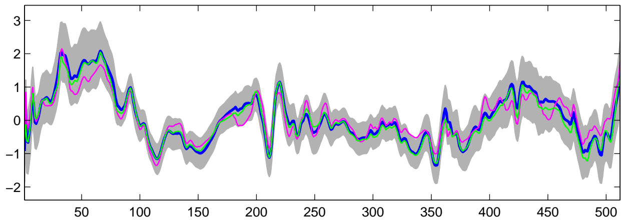
Estimated U_5(t) using G-WFMM: t_3 data, run 7
