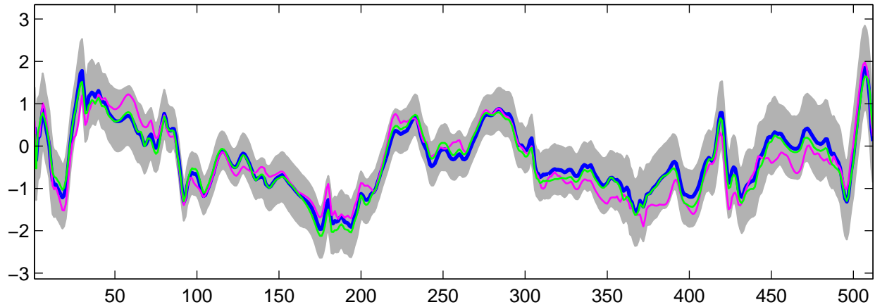
Estimated U_6(t) using G-WFMM: Normal data, run 7
