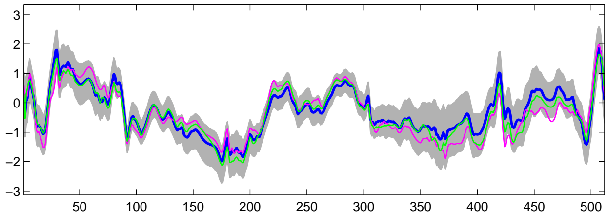
Estimated U_6(t) using R-WFMM: Normal data, run 7
